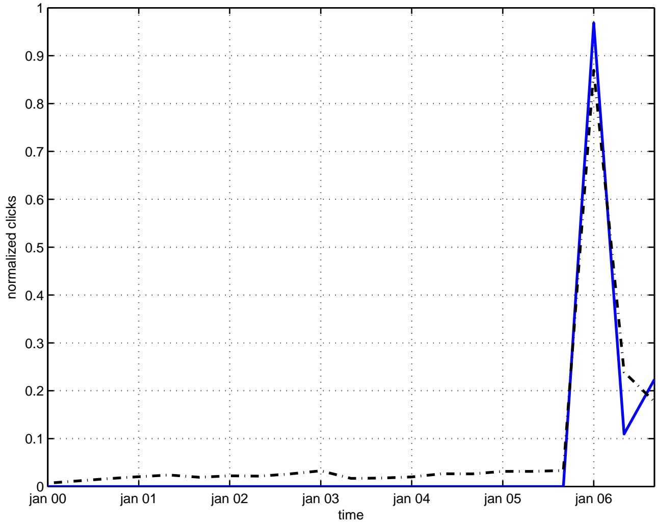
fock space boson
