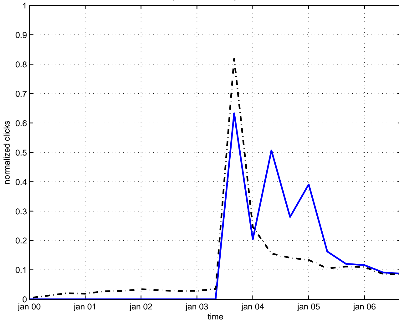
flux spontaneous compactification
