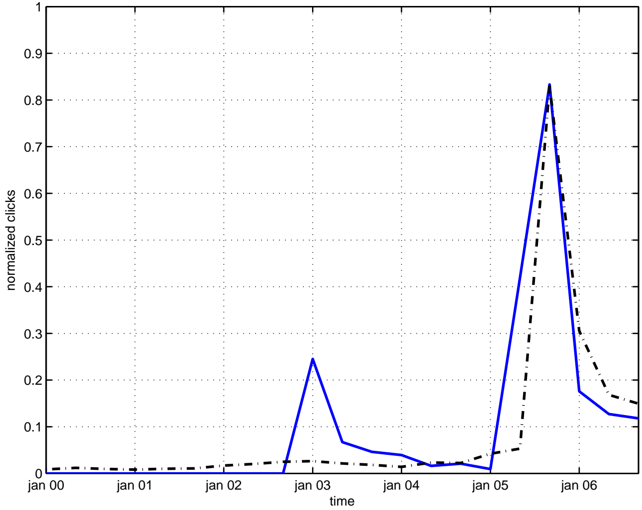
flux quantization
