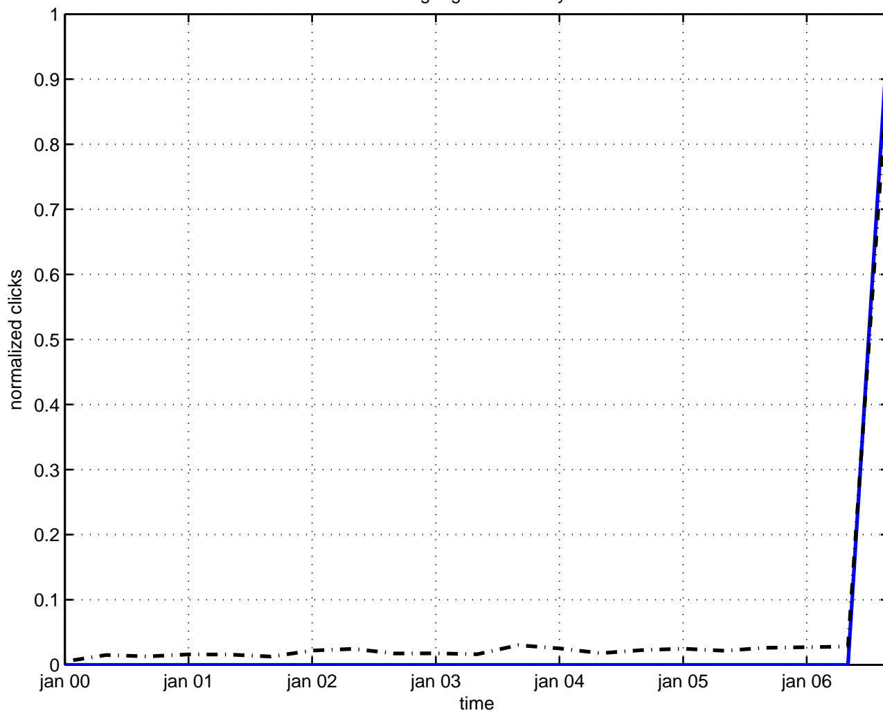
flux gauge field theory
