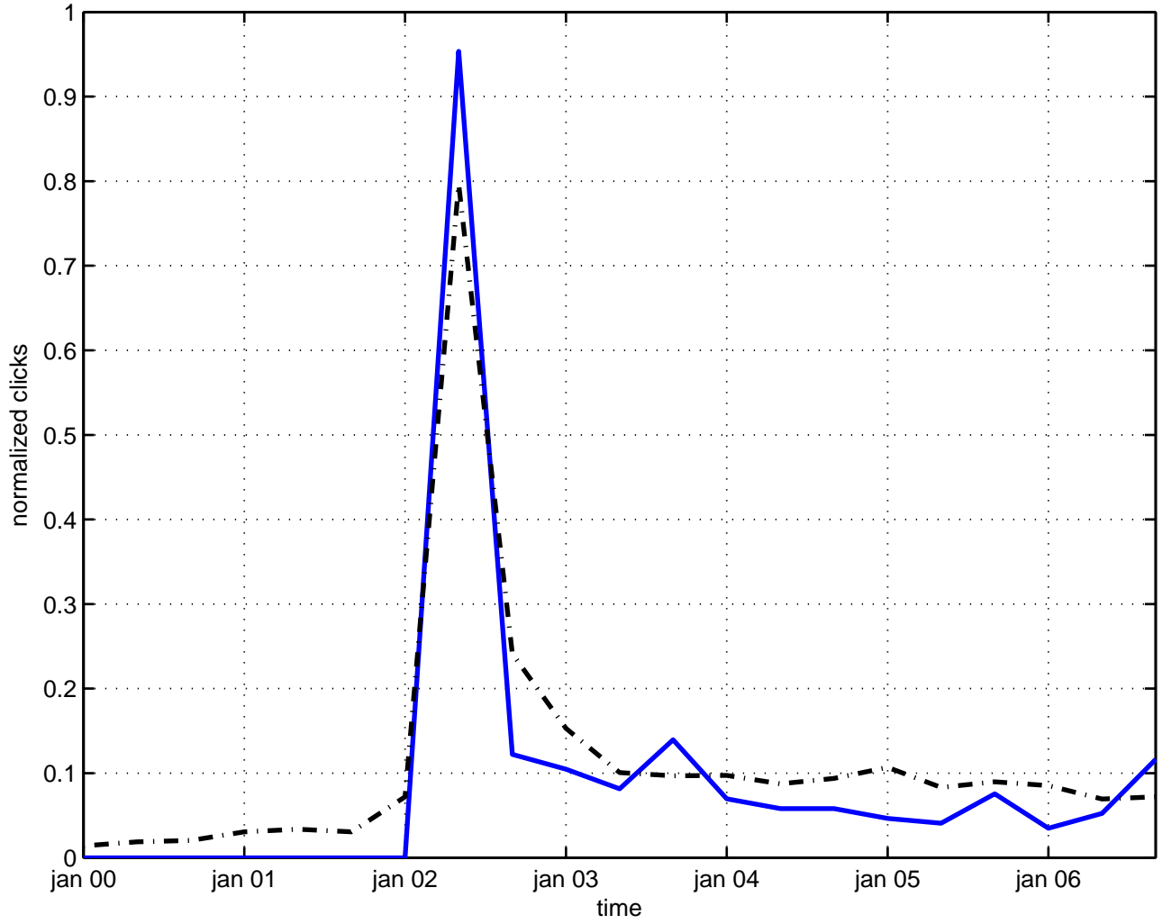
flux condensation
