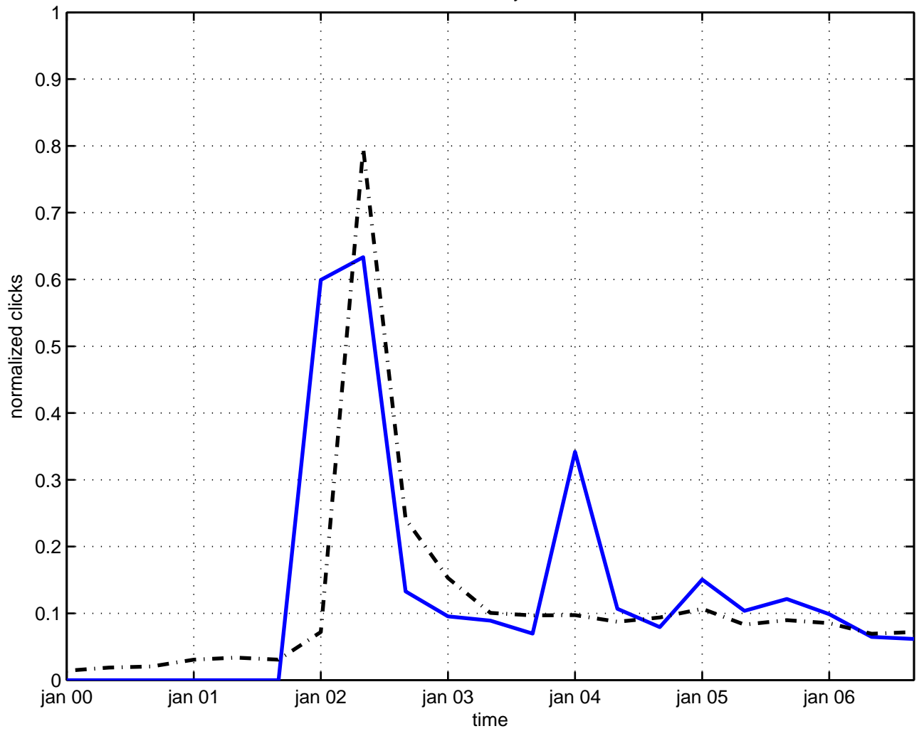
fluid tachyon
