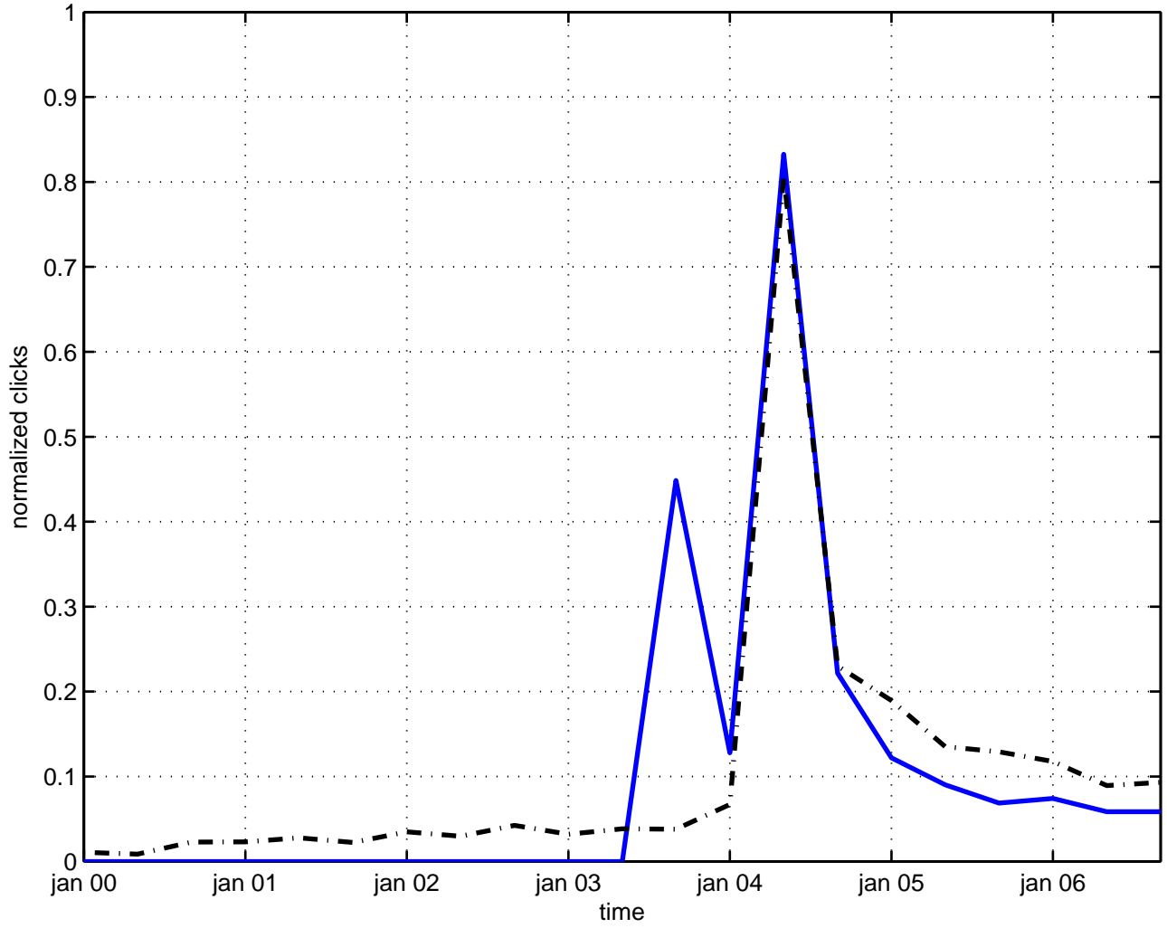
fluid black hole
