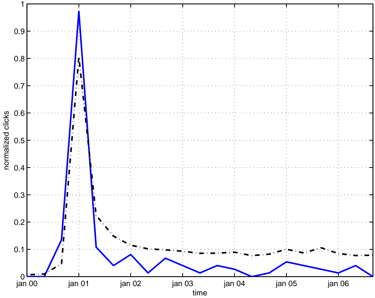
fluctuation vertex
