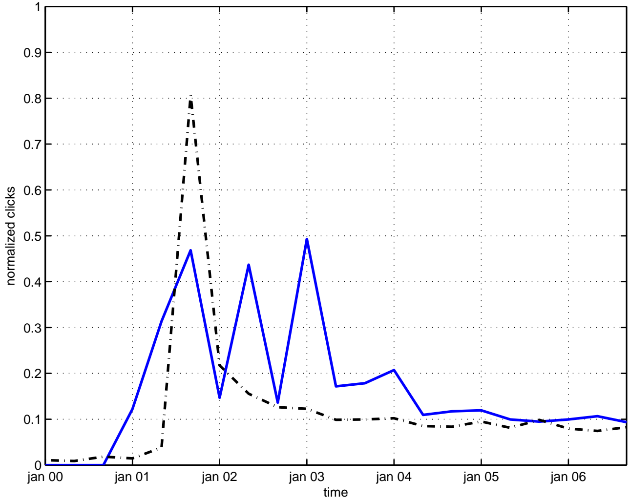
fluctuation thermodynamics
