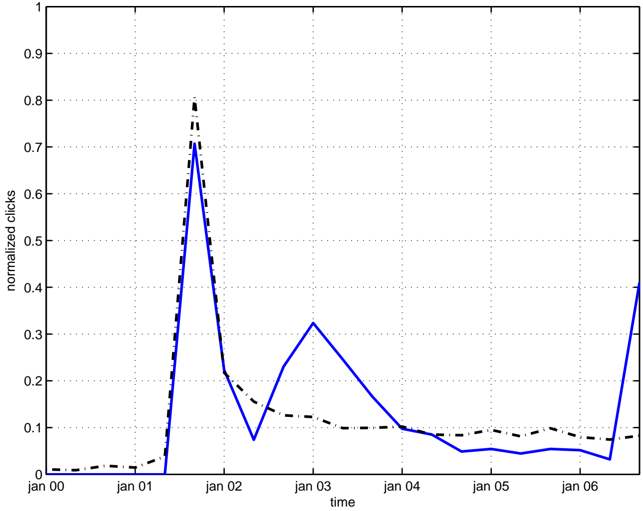
fluctuation tachyon
