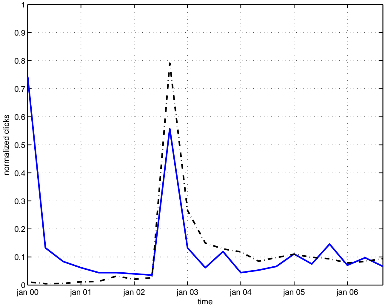
fluctuation string model
