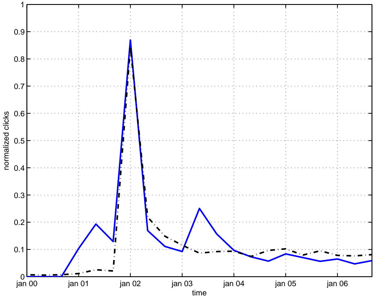
fluctuation spectrum
