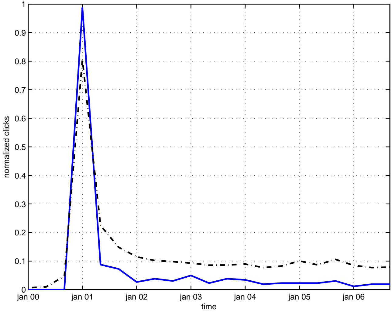
fluctuation soliton
