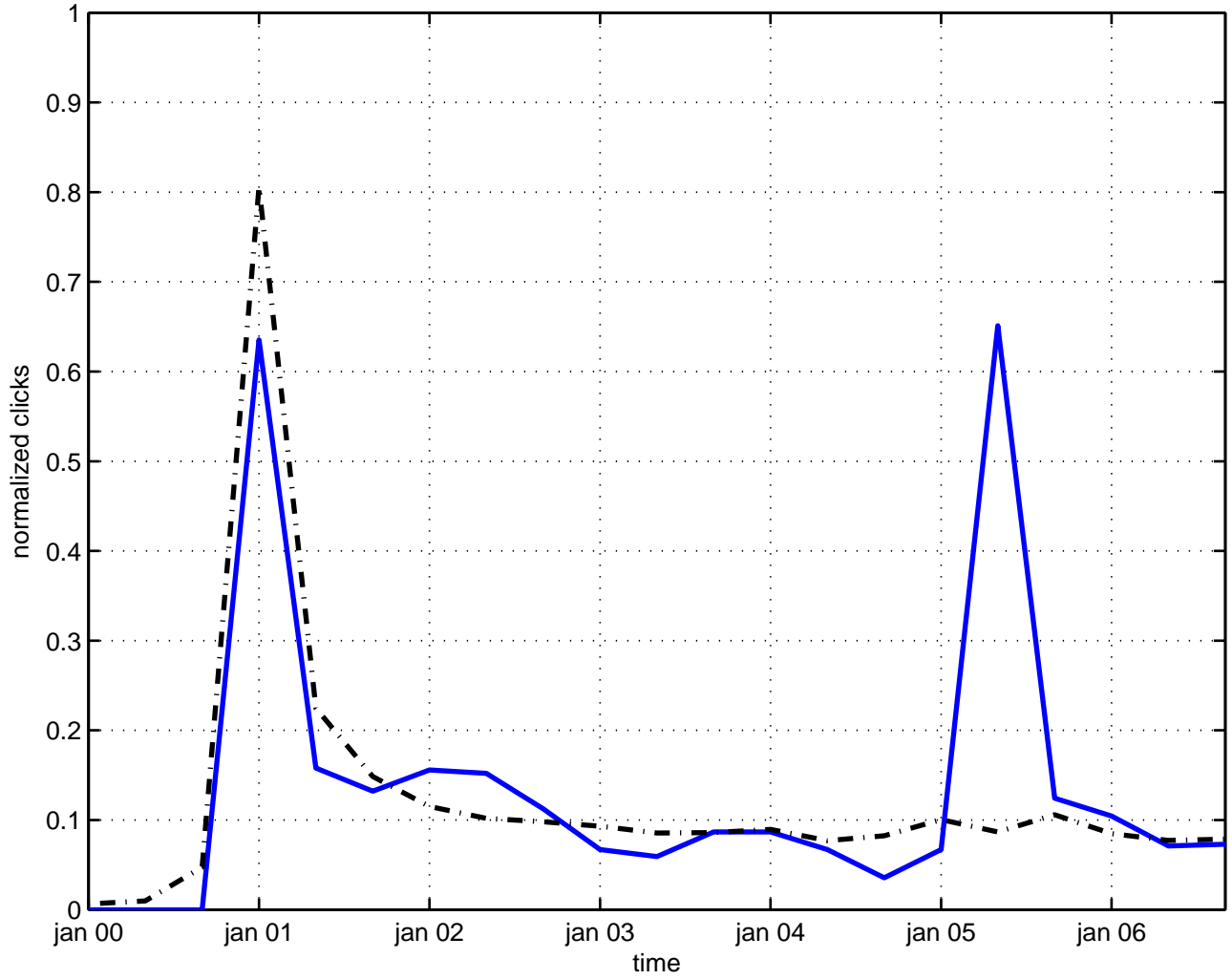
fluctuation radion
