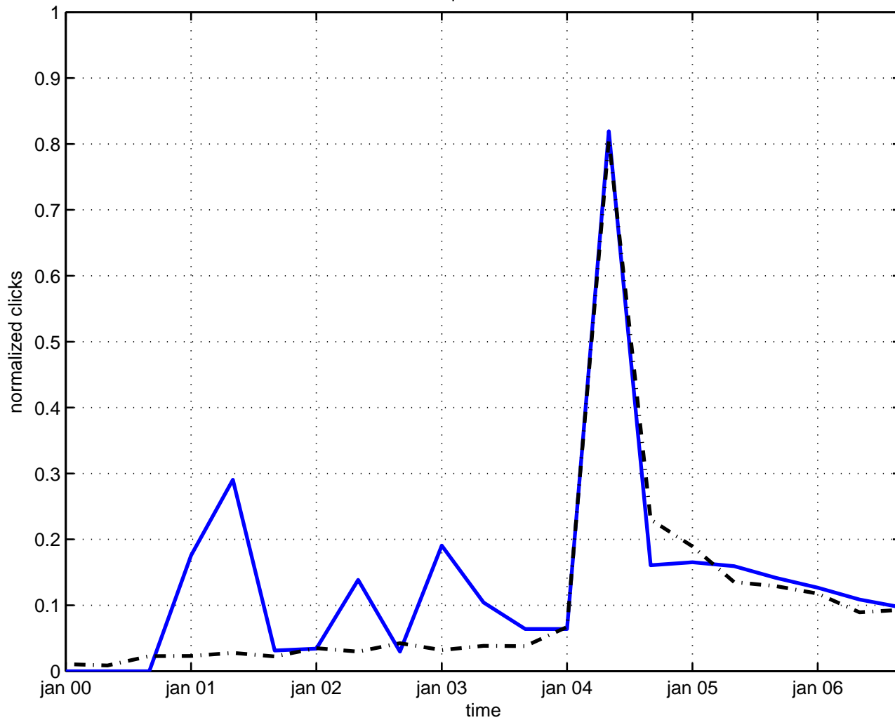
fluctuation quantum mechanics
