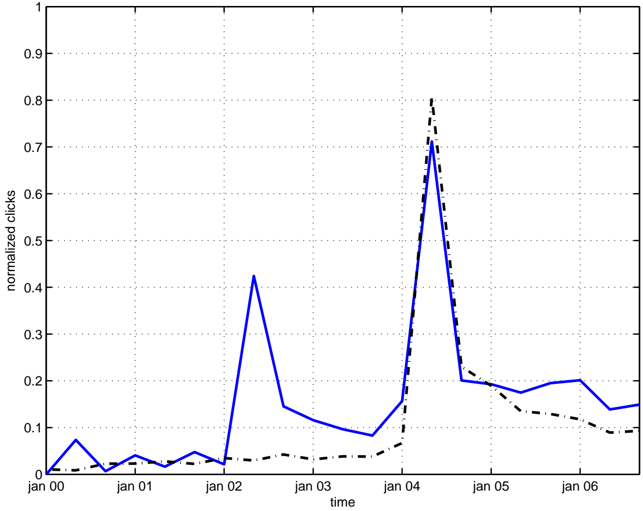
fluctuation quantization
