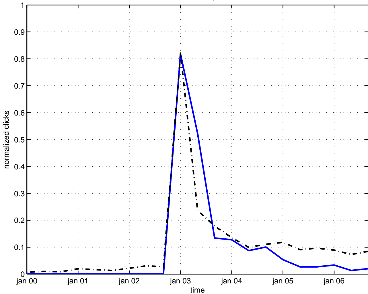
fluctuation pi
