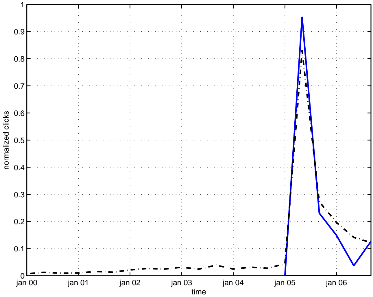
fluctuation phase
