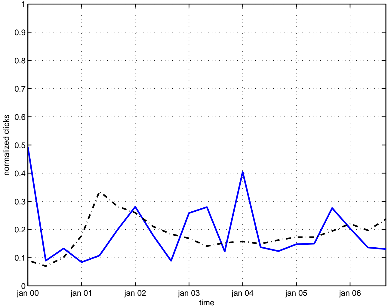
fluctuation gravitation
