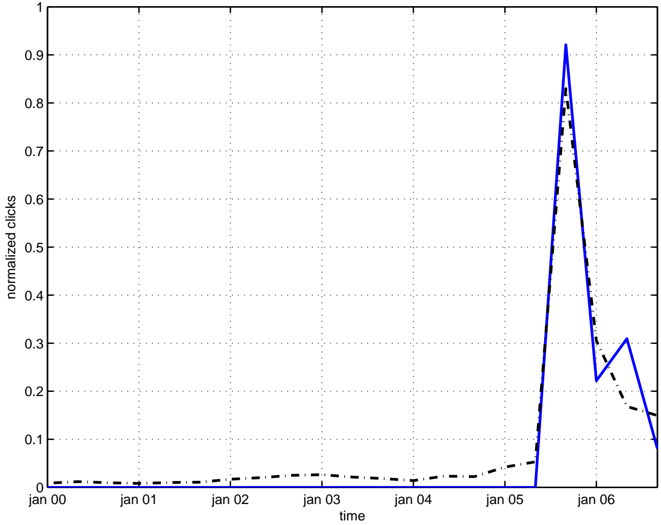
fluctuation axion
