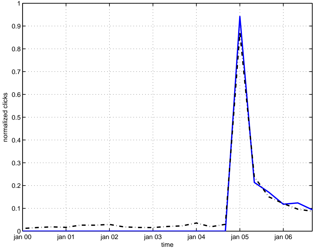
fixed point stability
