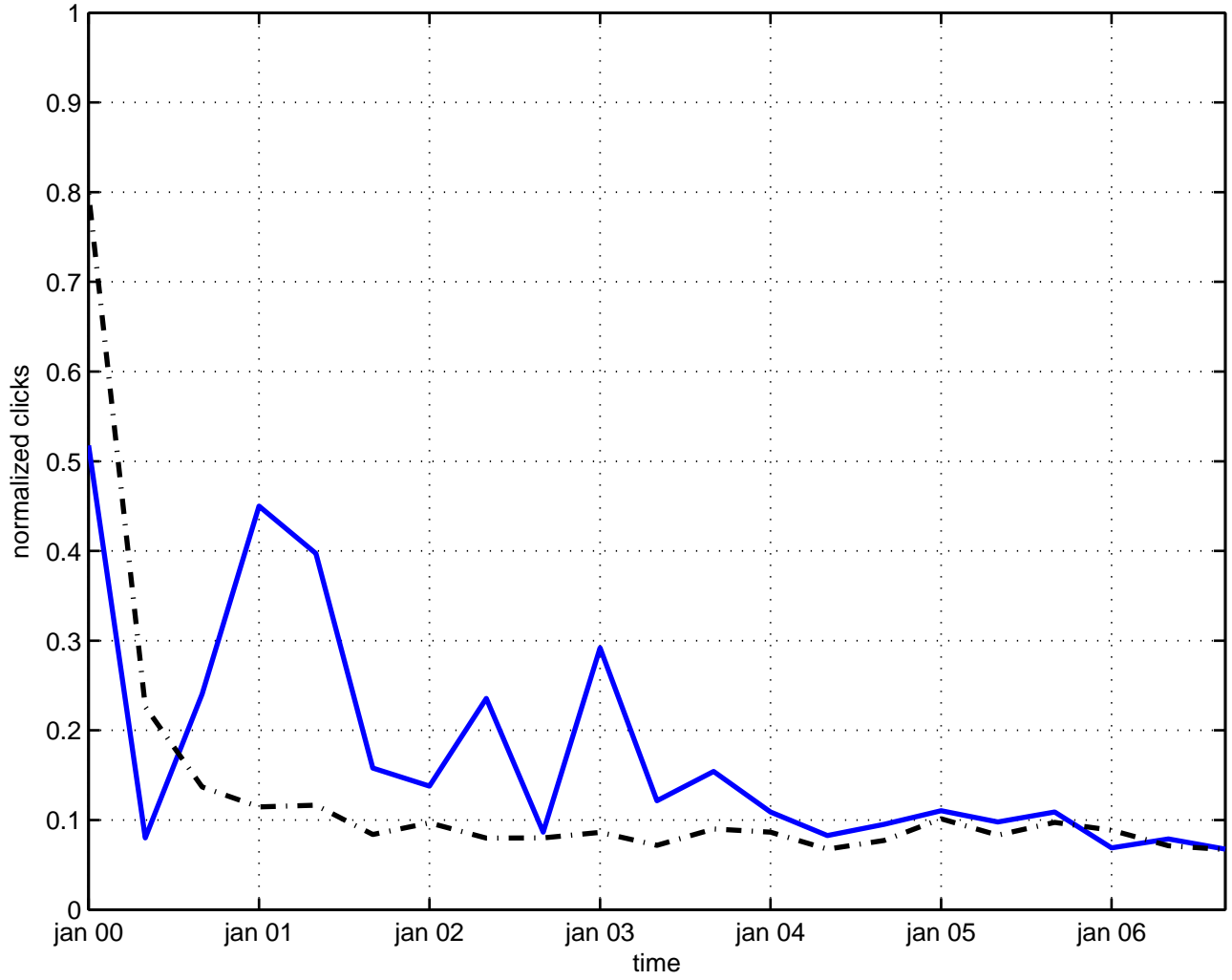
fixed point infrared problem
