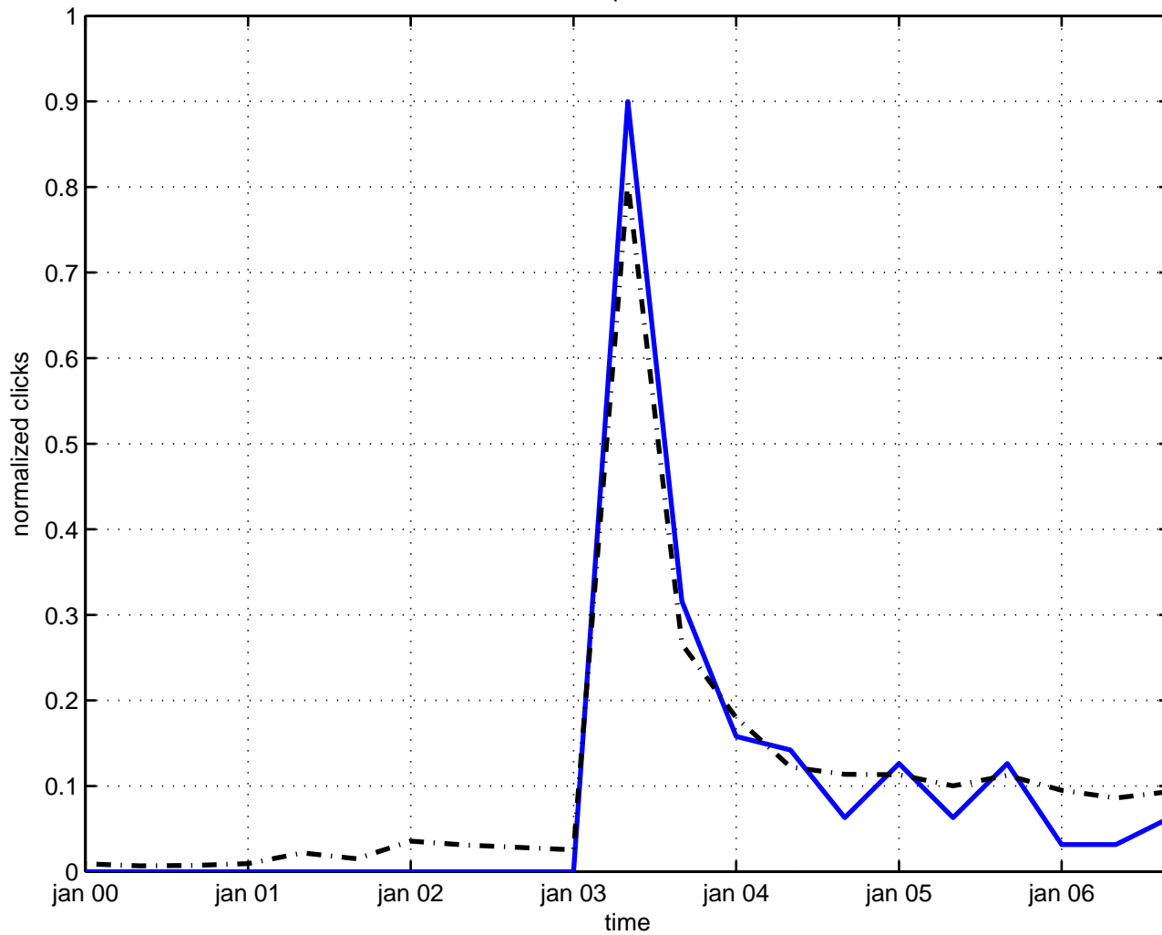
finsler space-time
