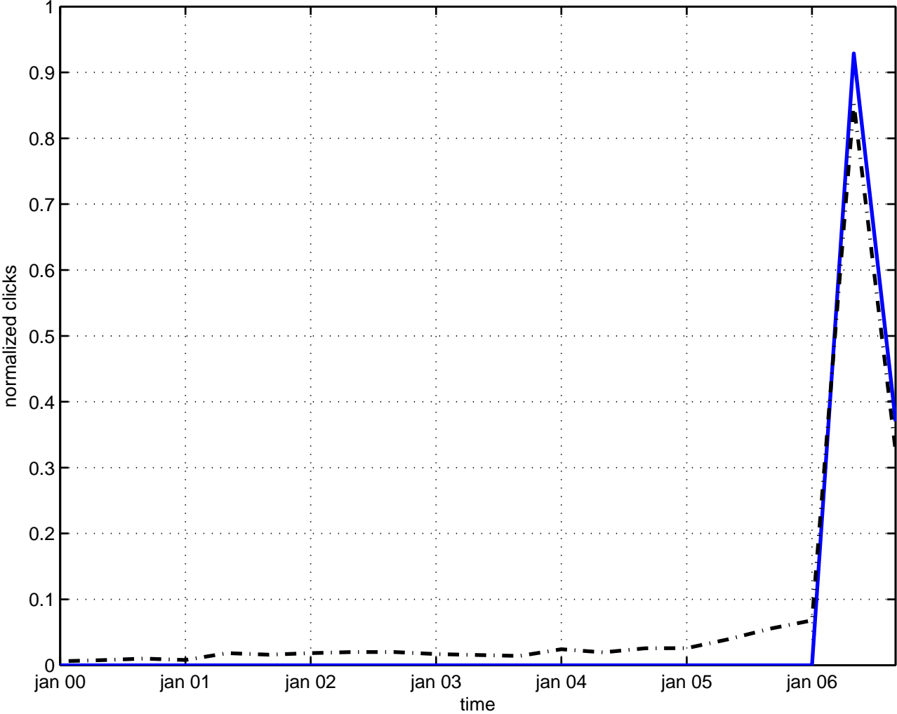
finite temperature gauge field theory
