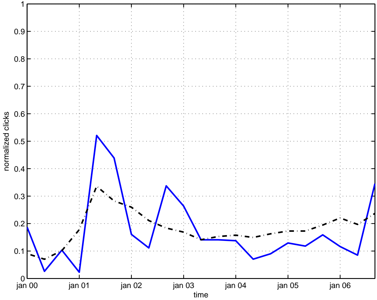
finite temperature field theory
