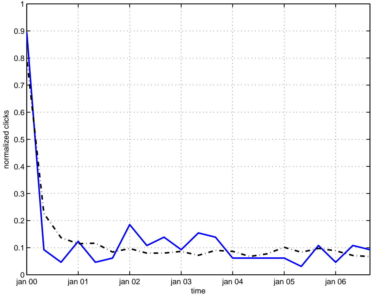
finite space-time
