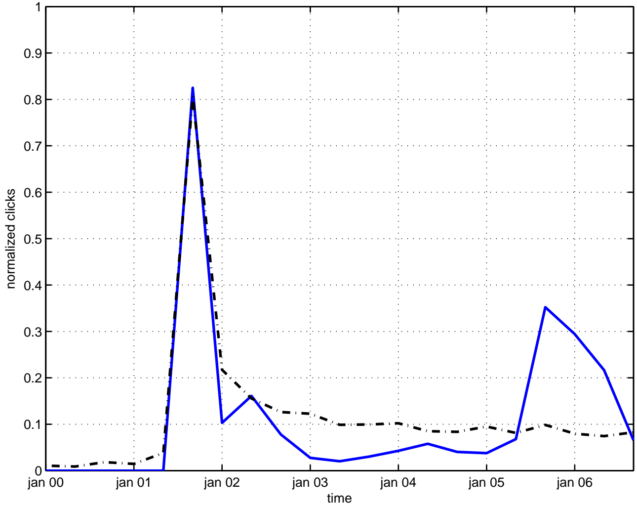
finite scattering amplitude
