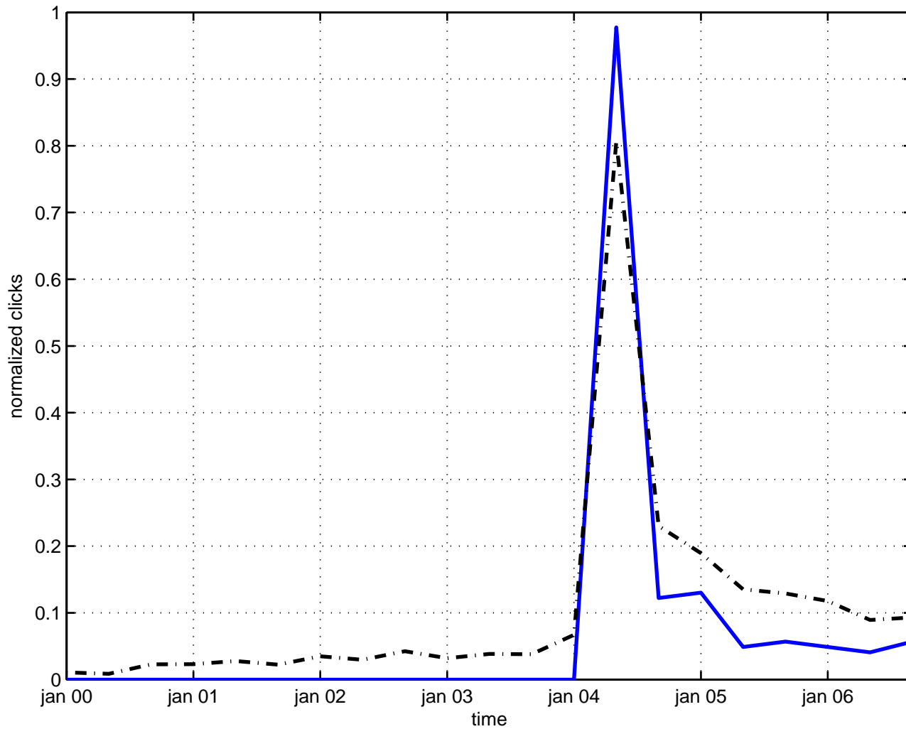
finite s-matrix
