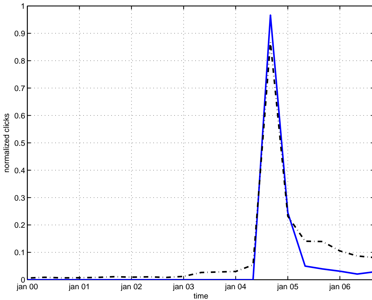
finite renormalization
