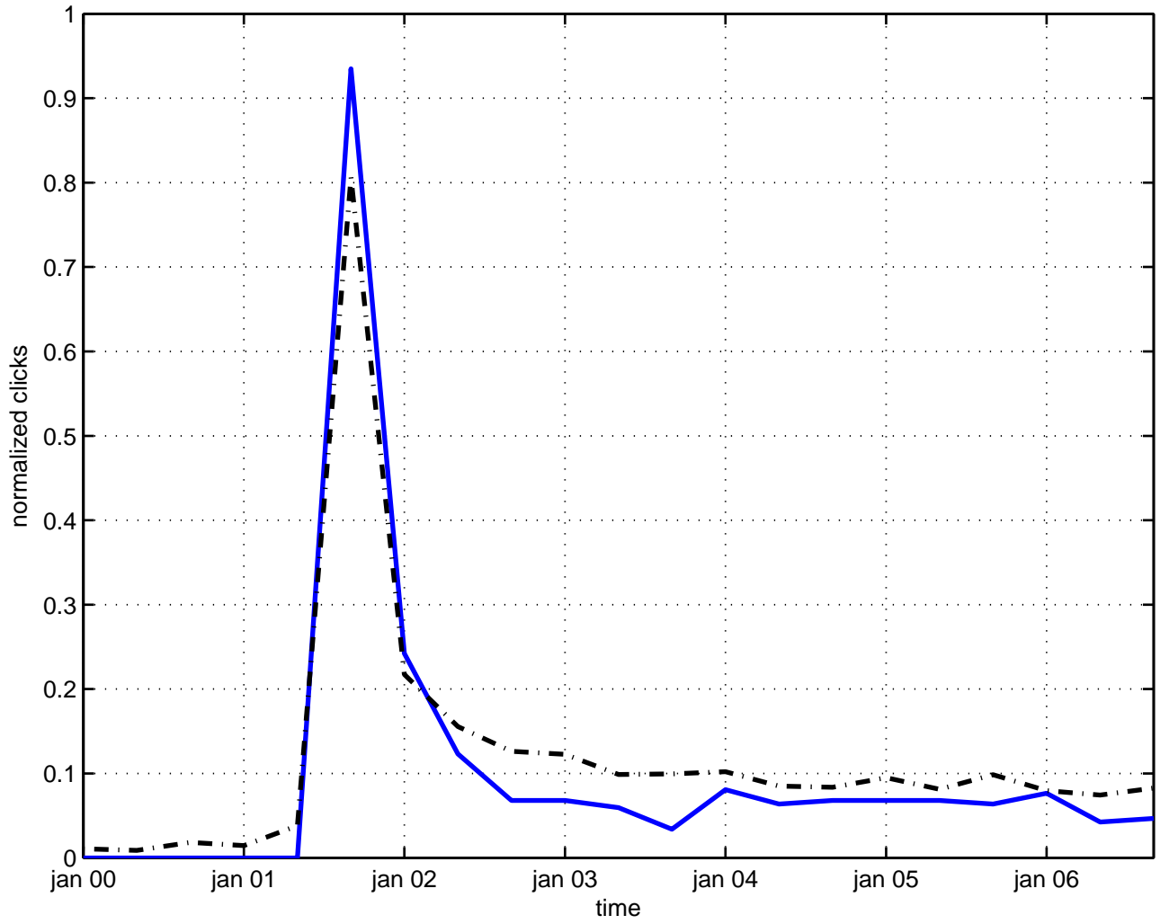
finite m-theory
