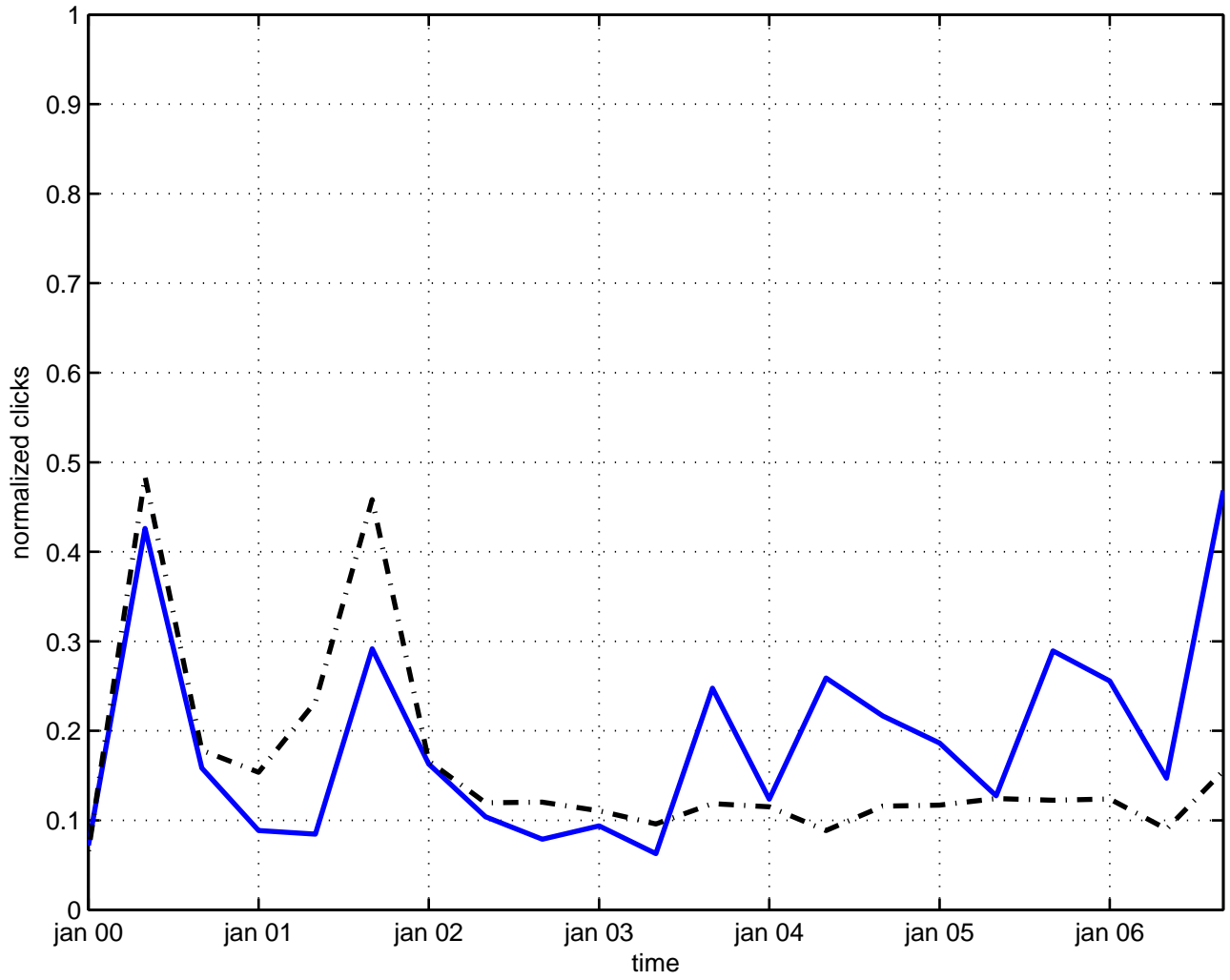
finite group
