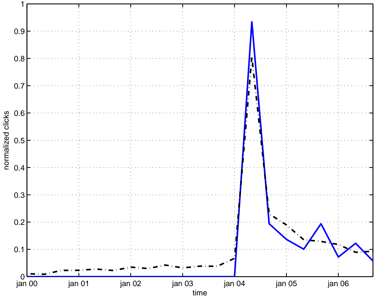
finite gauge field theory
