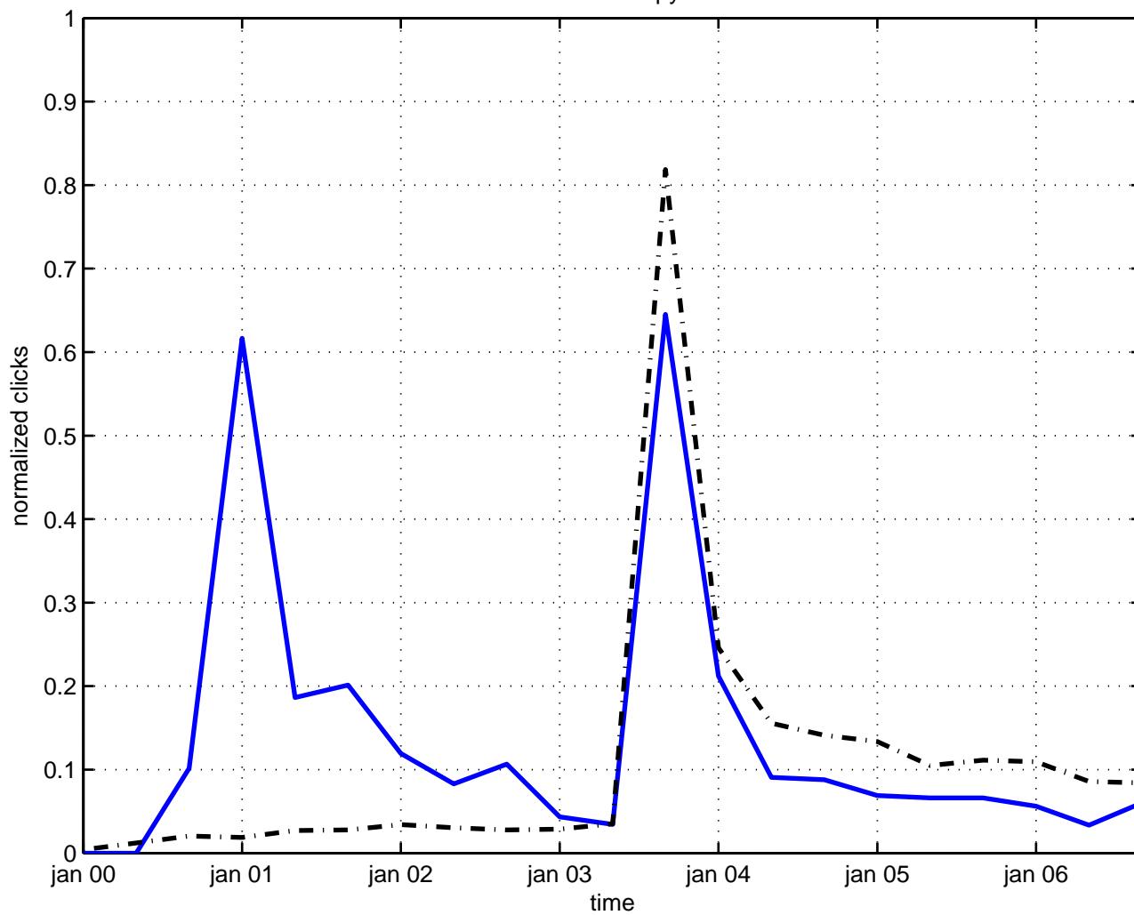
finite entropy
