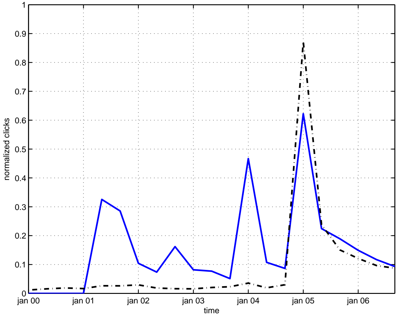
finite energy
