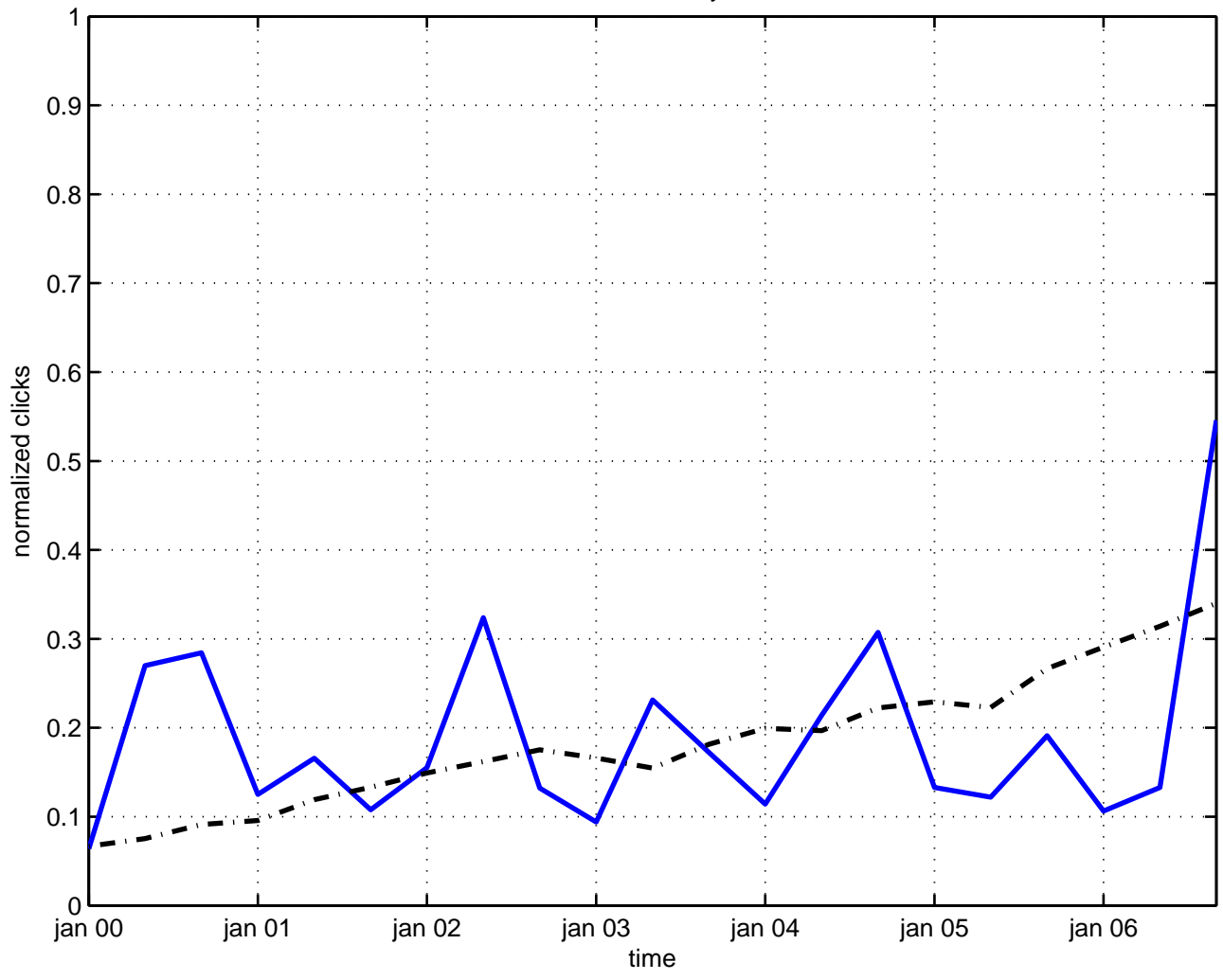
finite density
