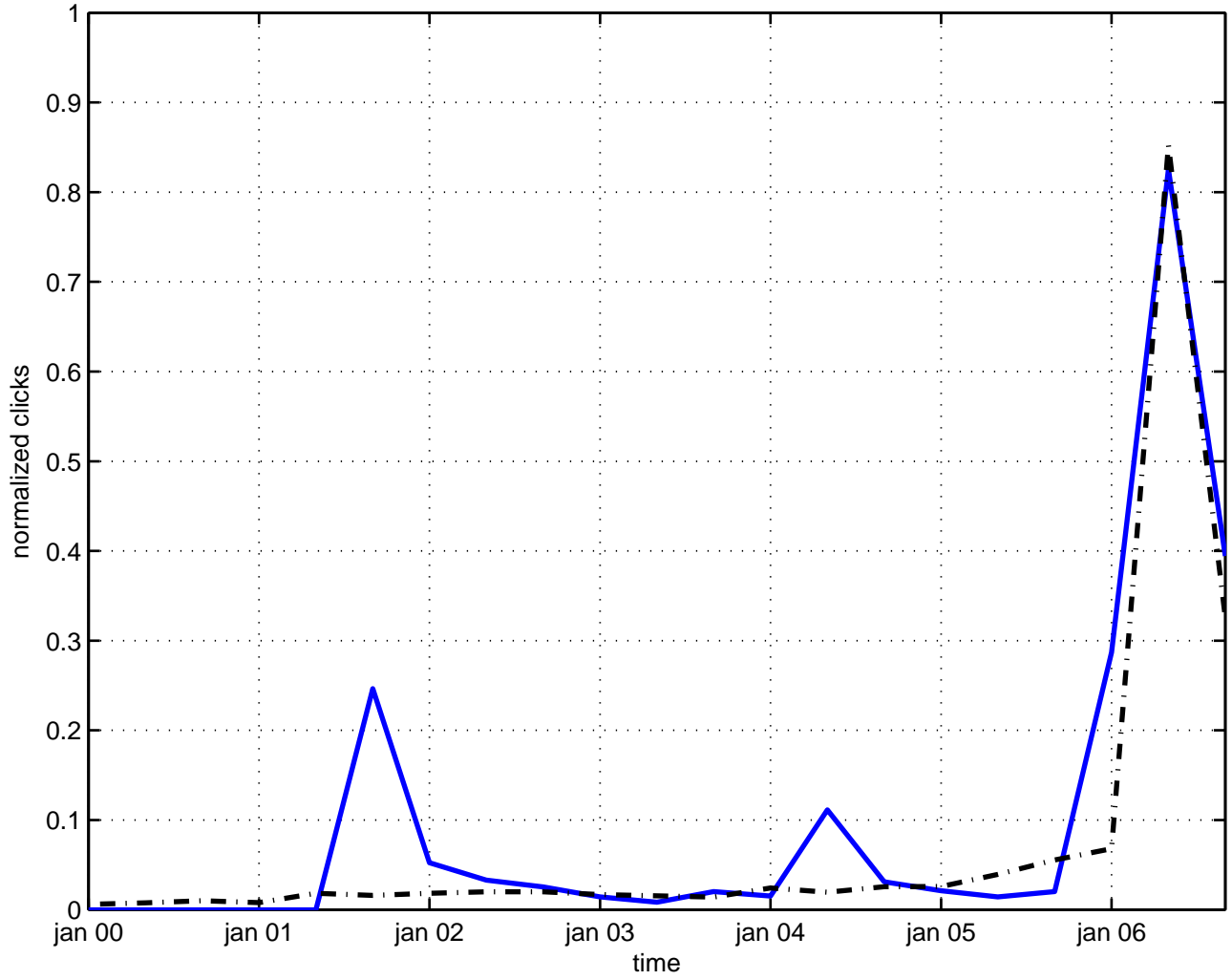
fifth force
