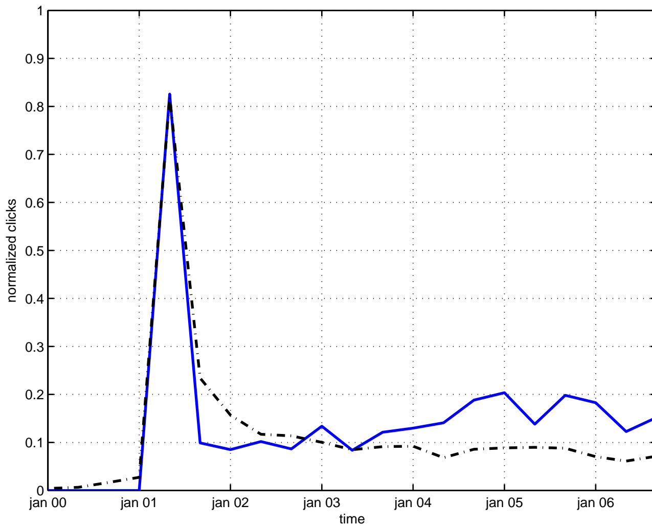
fierz transformation
