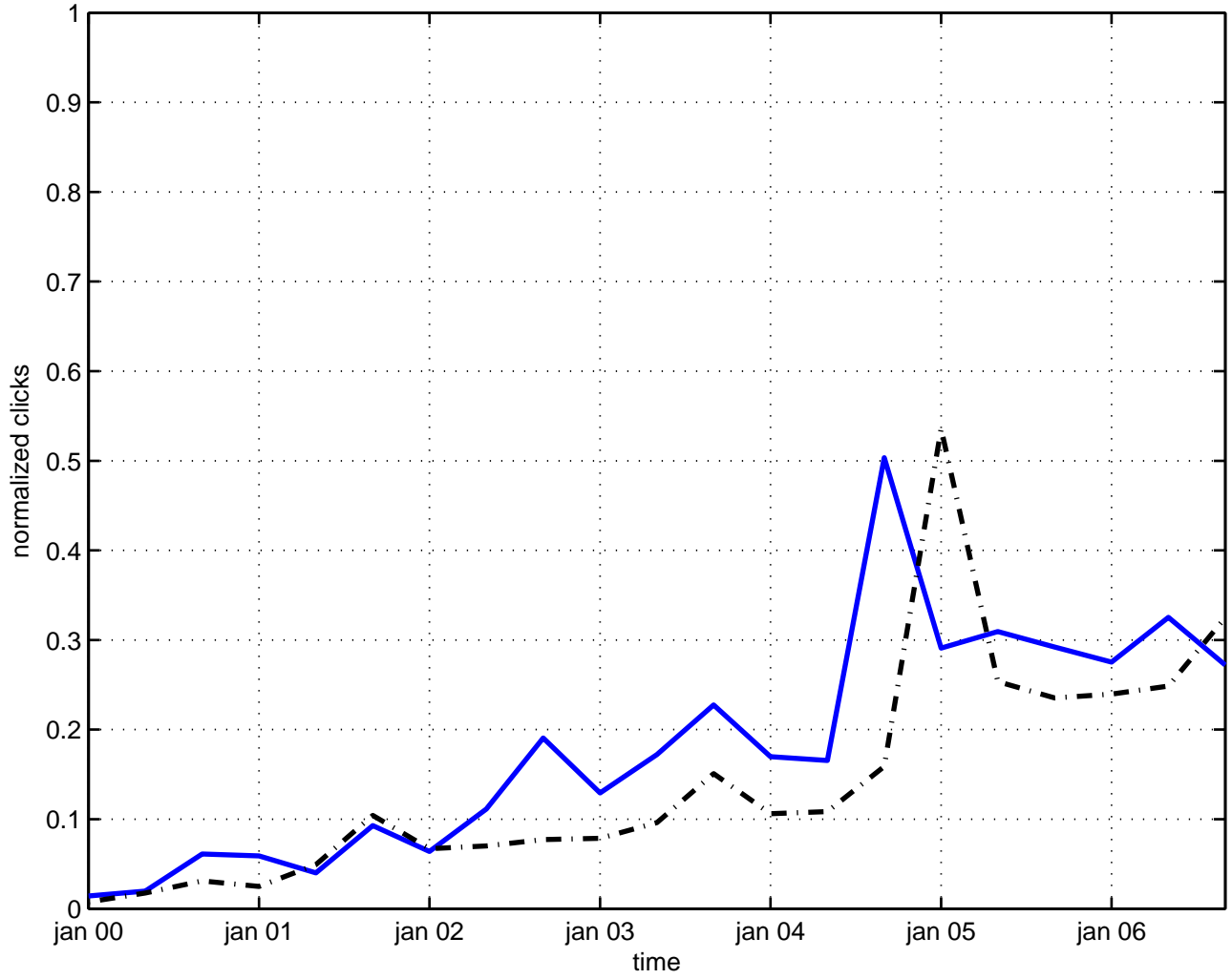
field theory
