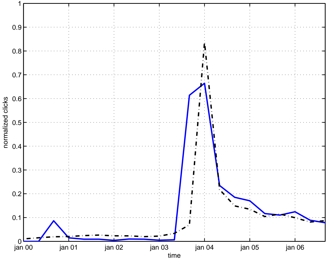
ferromagnet model
