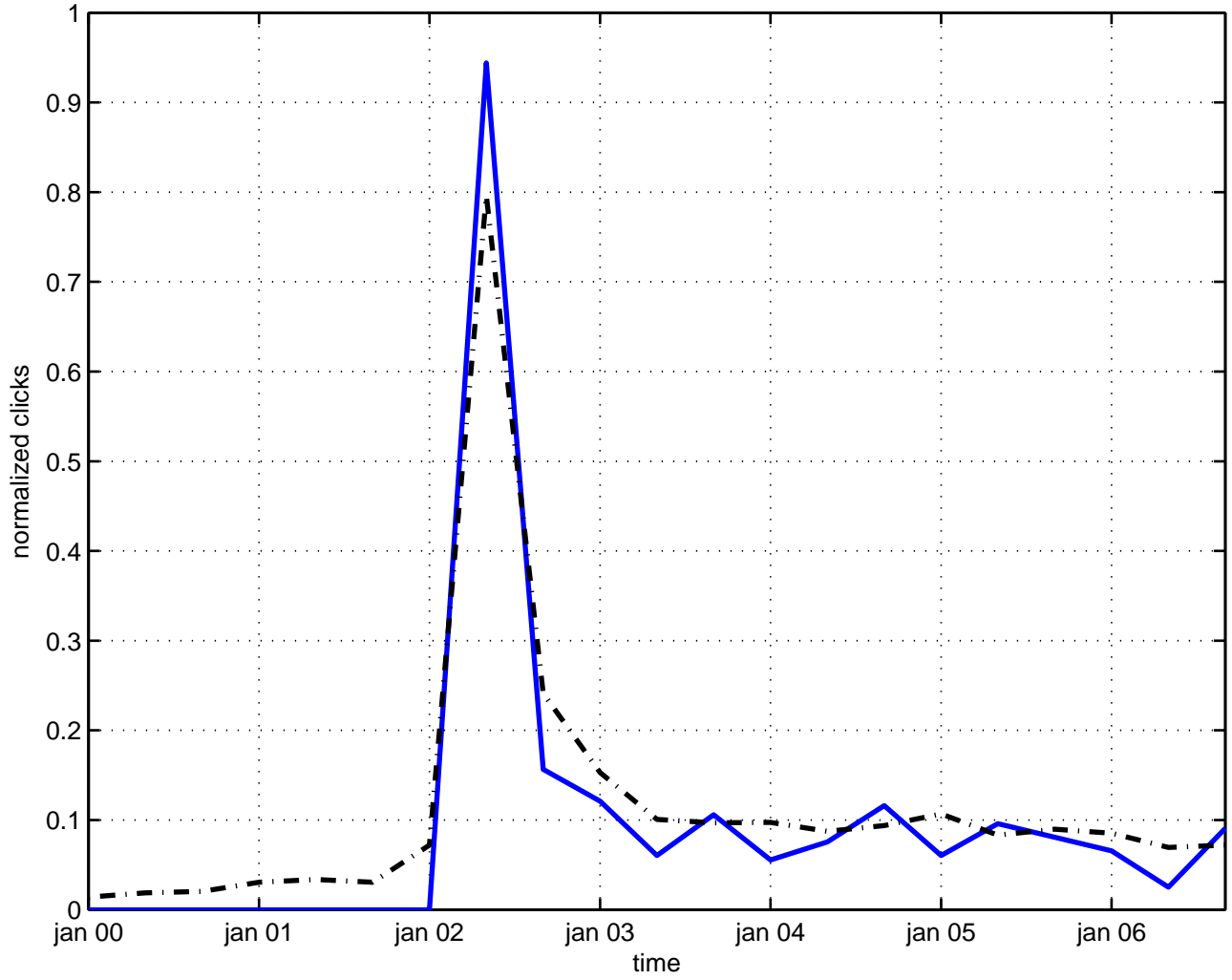
factorization zero mode
