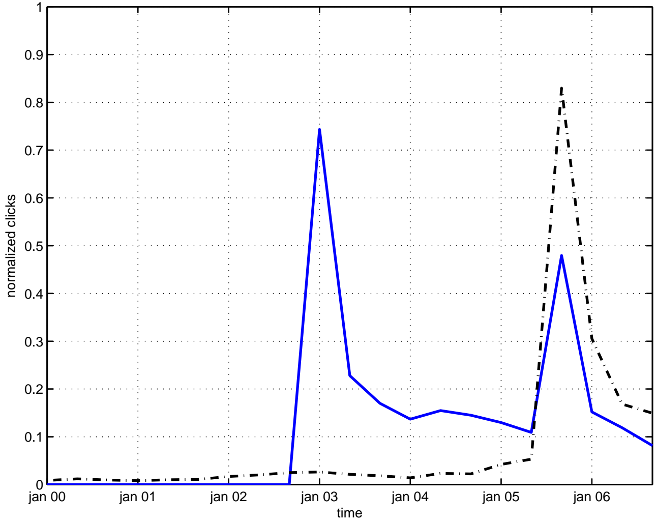
factorization space-time
