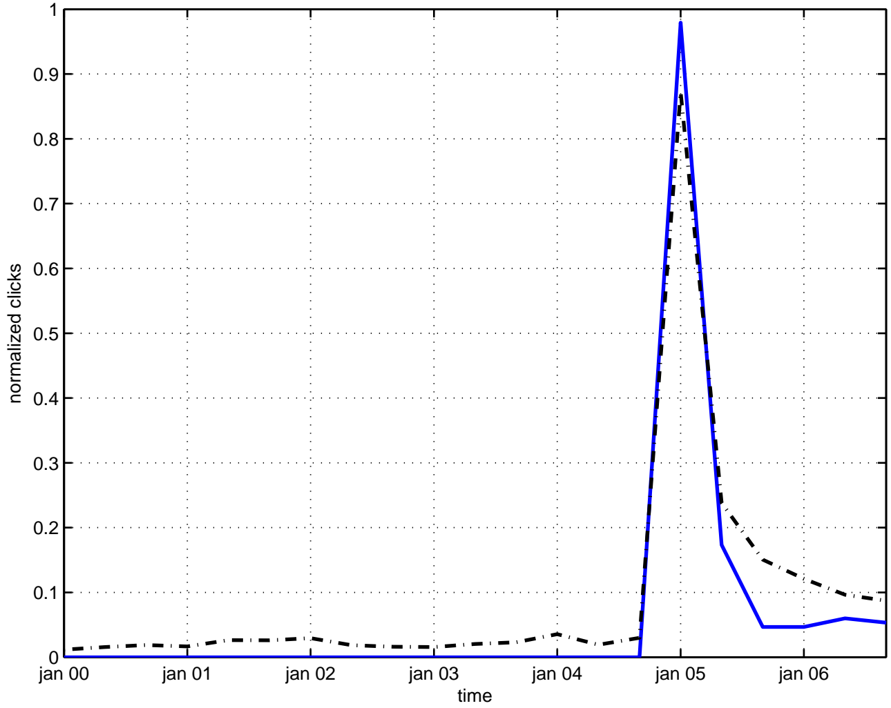
factorization path integral
