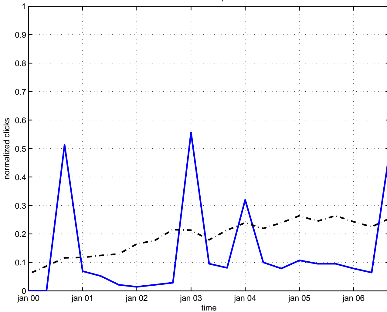
factorization operator
