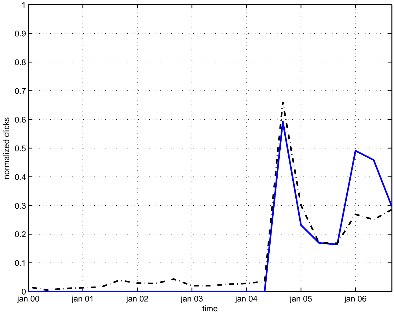
factorization matrix model
