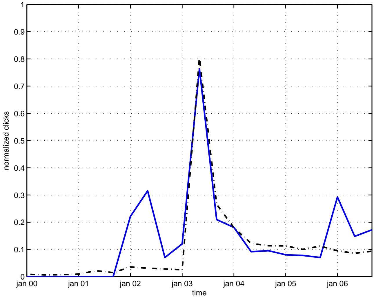
factorization algebra
