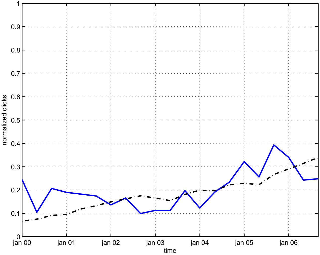
f-theory
