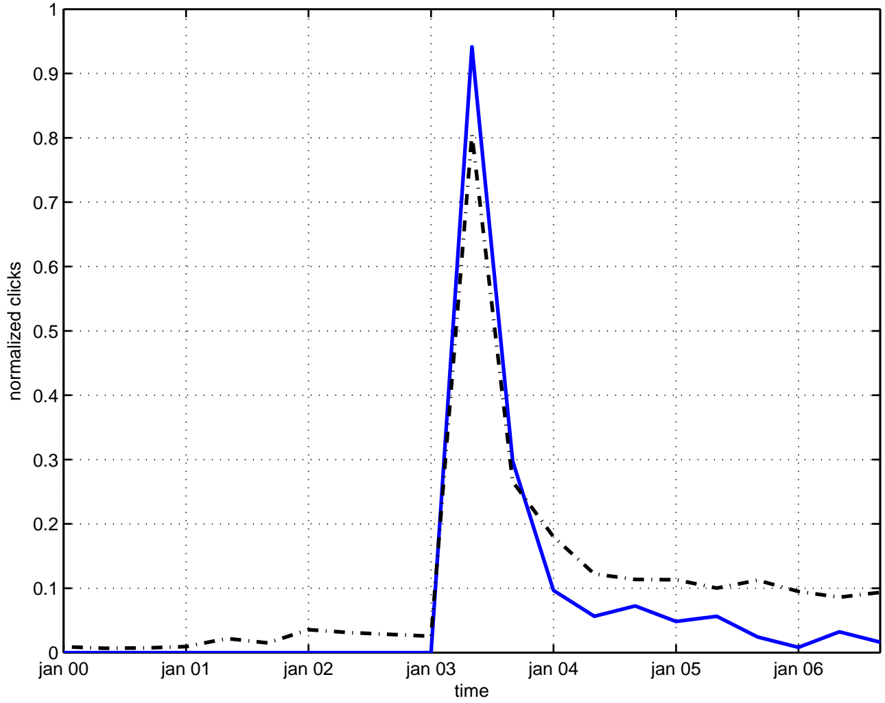
f-term gauge field theory
