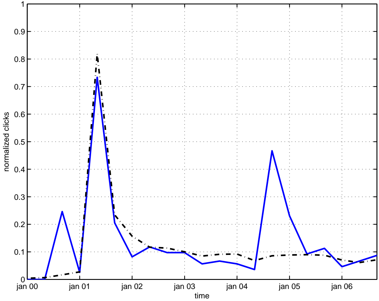
f(4) algebra
