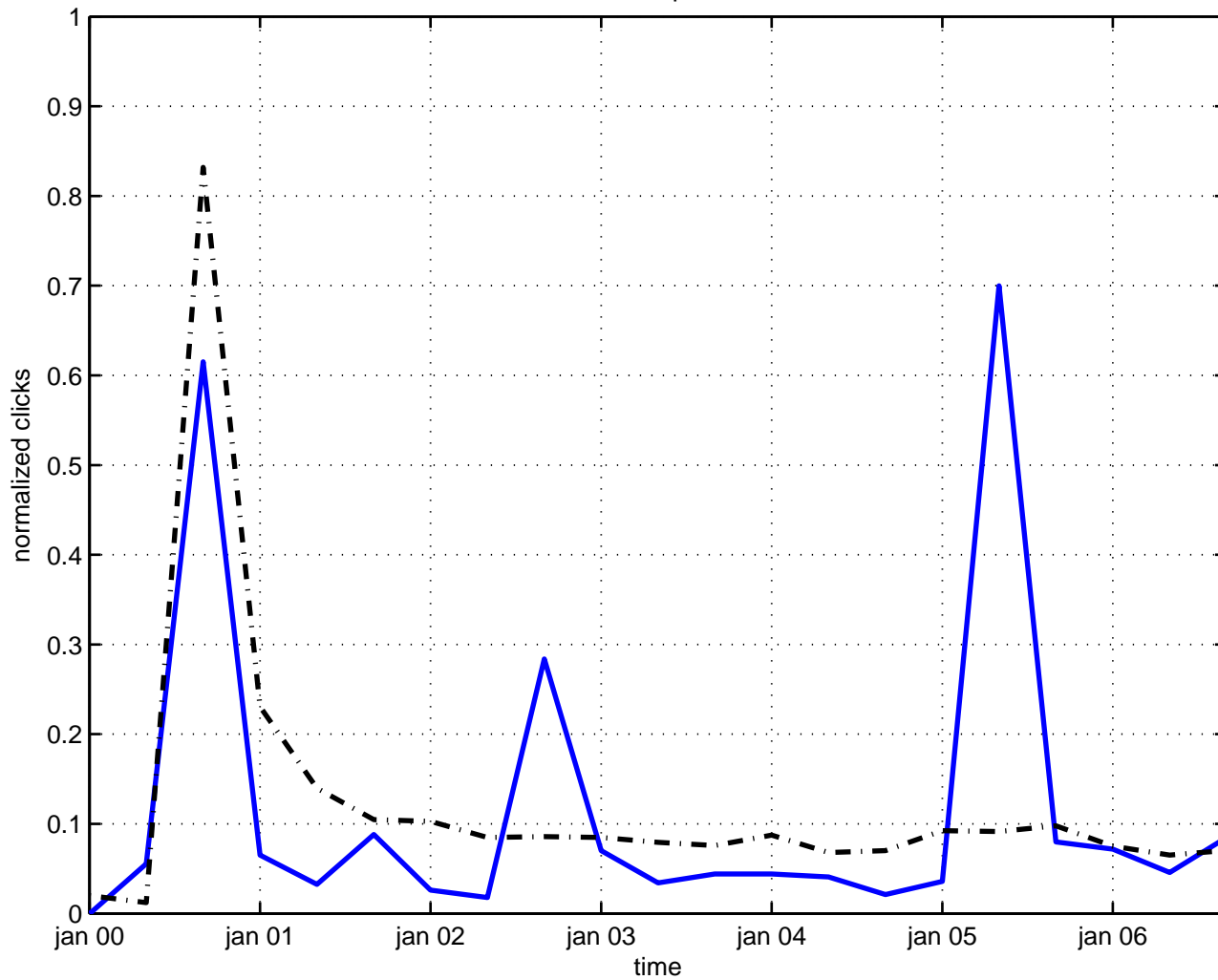
extended particle
