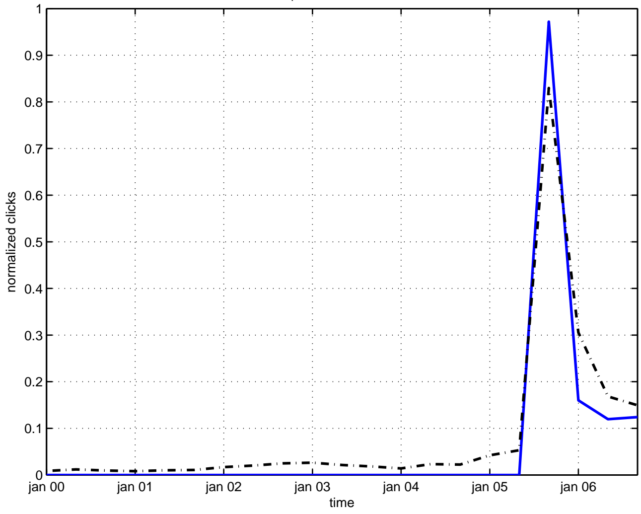
expansion momentum
